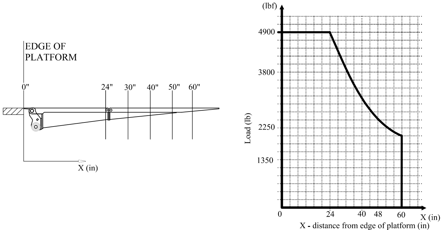
Figure 1 : F3RE49 Load Capacity
