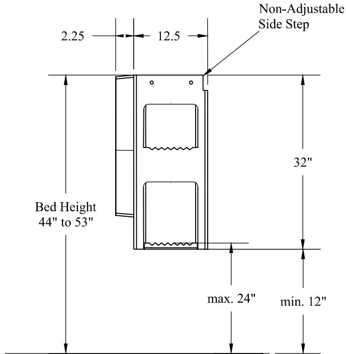
Figure 3 : REP 33 Side Step
