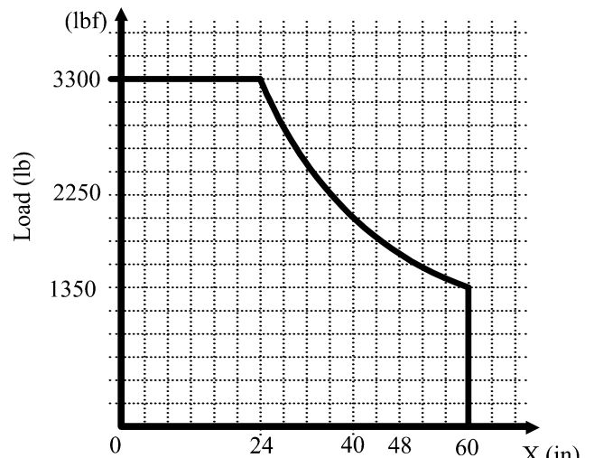
Figure 1: REP 33/1 Load Capacity X - distance from edge of platform (in)
