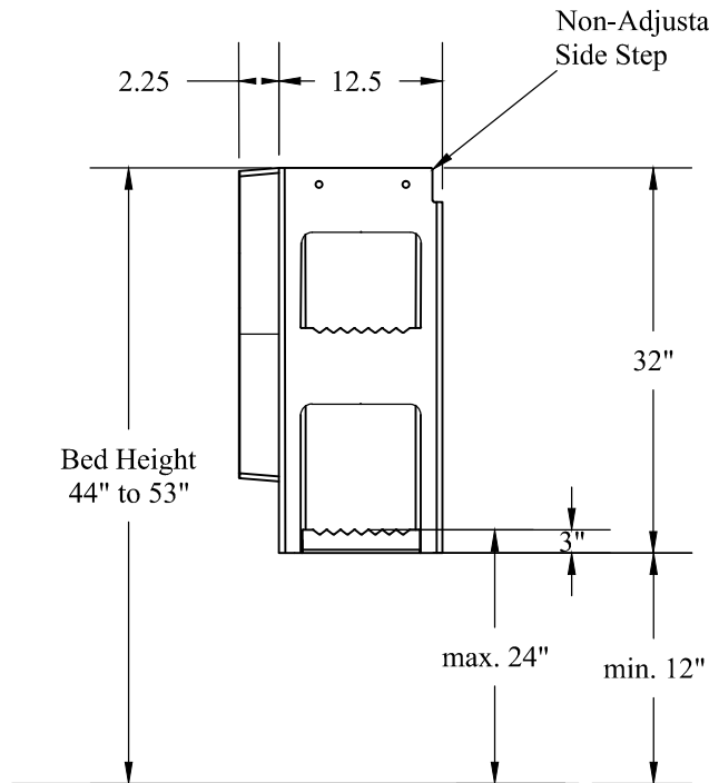
Figure 3 : REP 44/2 Side Step
