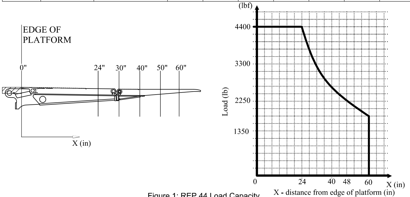
Figure 1: REP 44 Load Capacity
